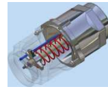
Pressure & Vacuum Relief valve
