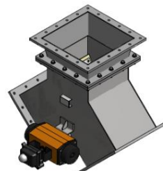
Gravity feed Diverter Valve
