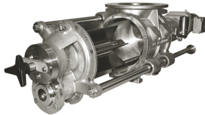
Blow Through Rotary valve / normal , quick detachable and dairy valve type
