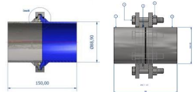
Self Aligning Flanges
