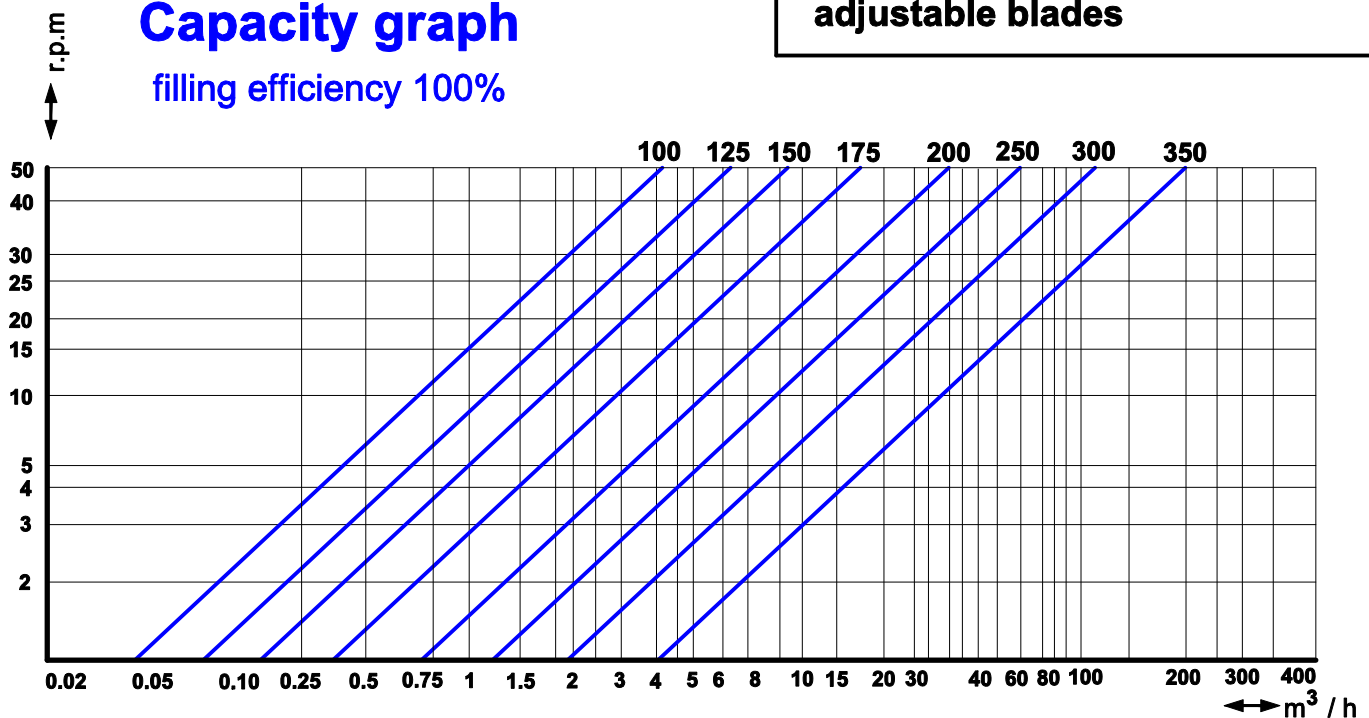
Rotor with replaceable and adjustable blades
